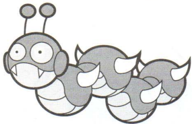
Caterkiller
